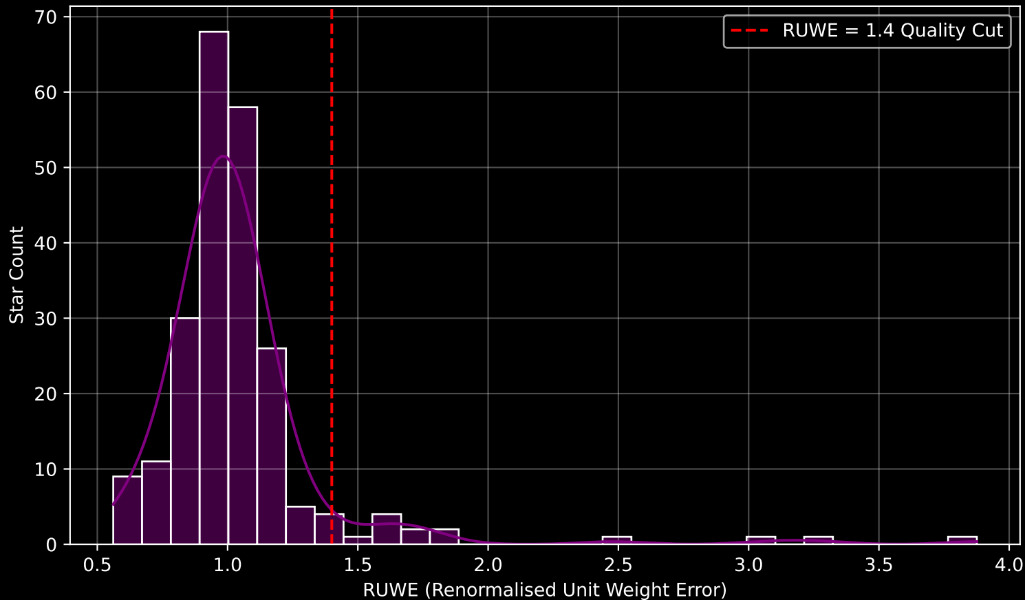
GAPOGEE DR17 Field [006-02] RUWE Distribution (n= 224)
