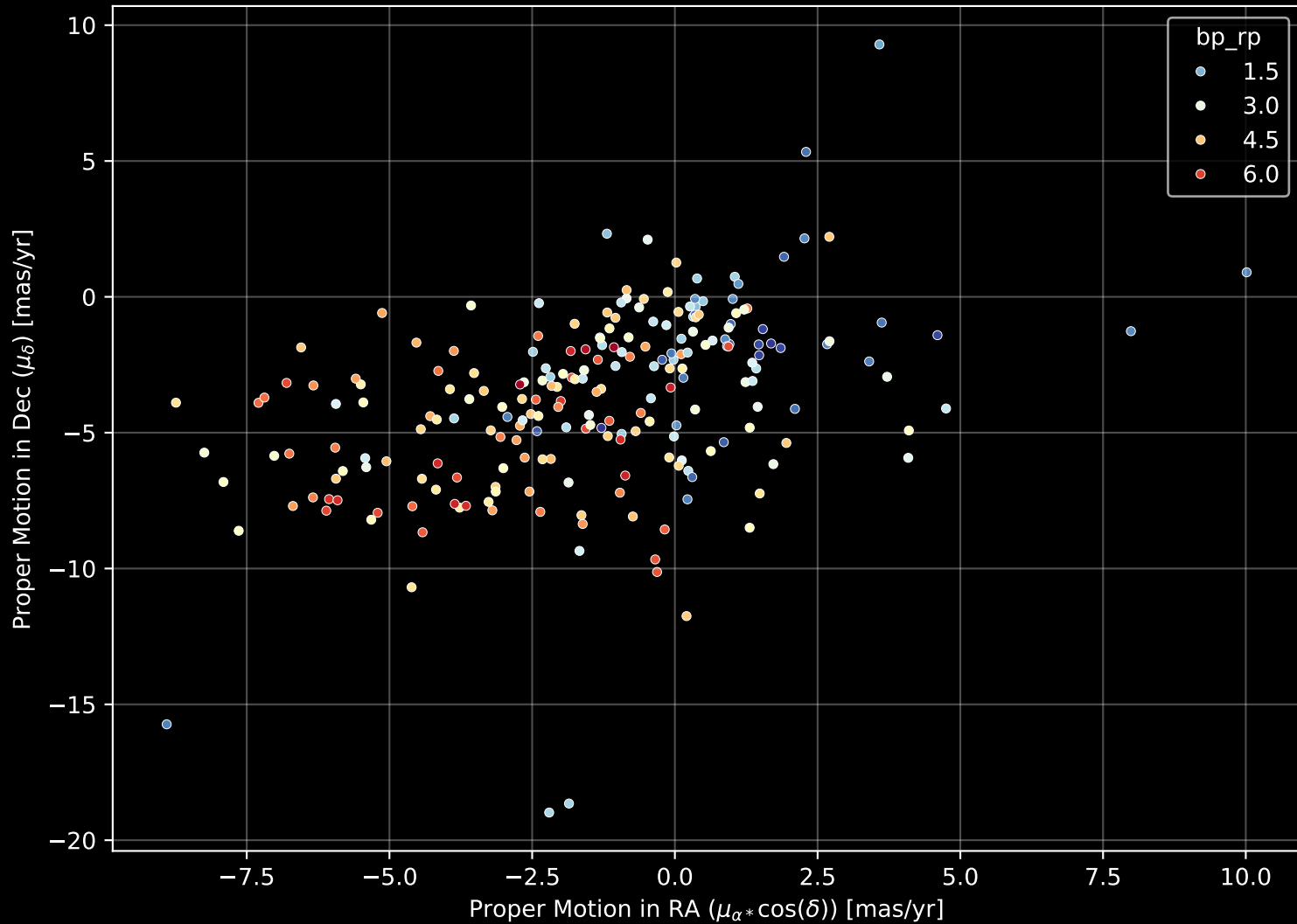
APOGEE DR17 Field: [006-02] Proper Motion Diagram (n= 225)
