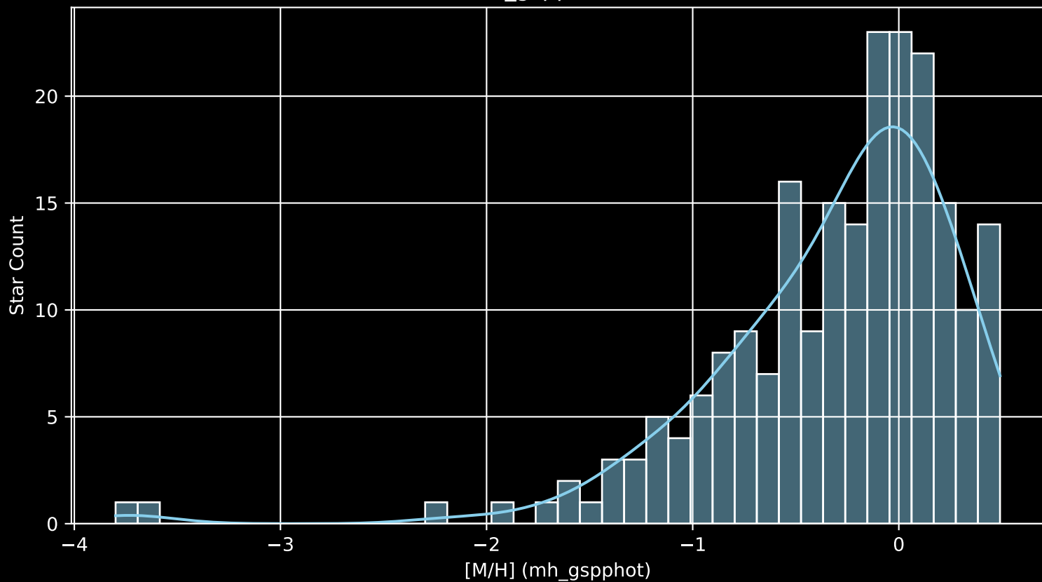
APOGEE DR17 Field: [006-02 [M/H] (mh_gspphot) (n= 214)
