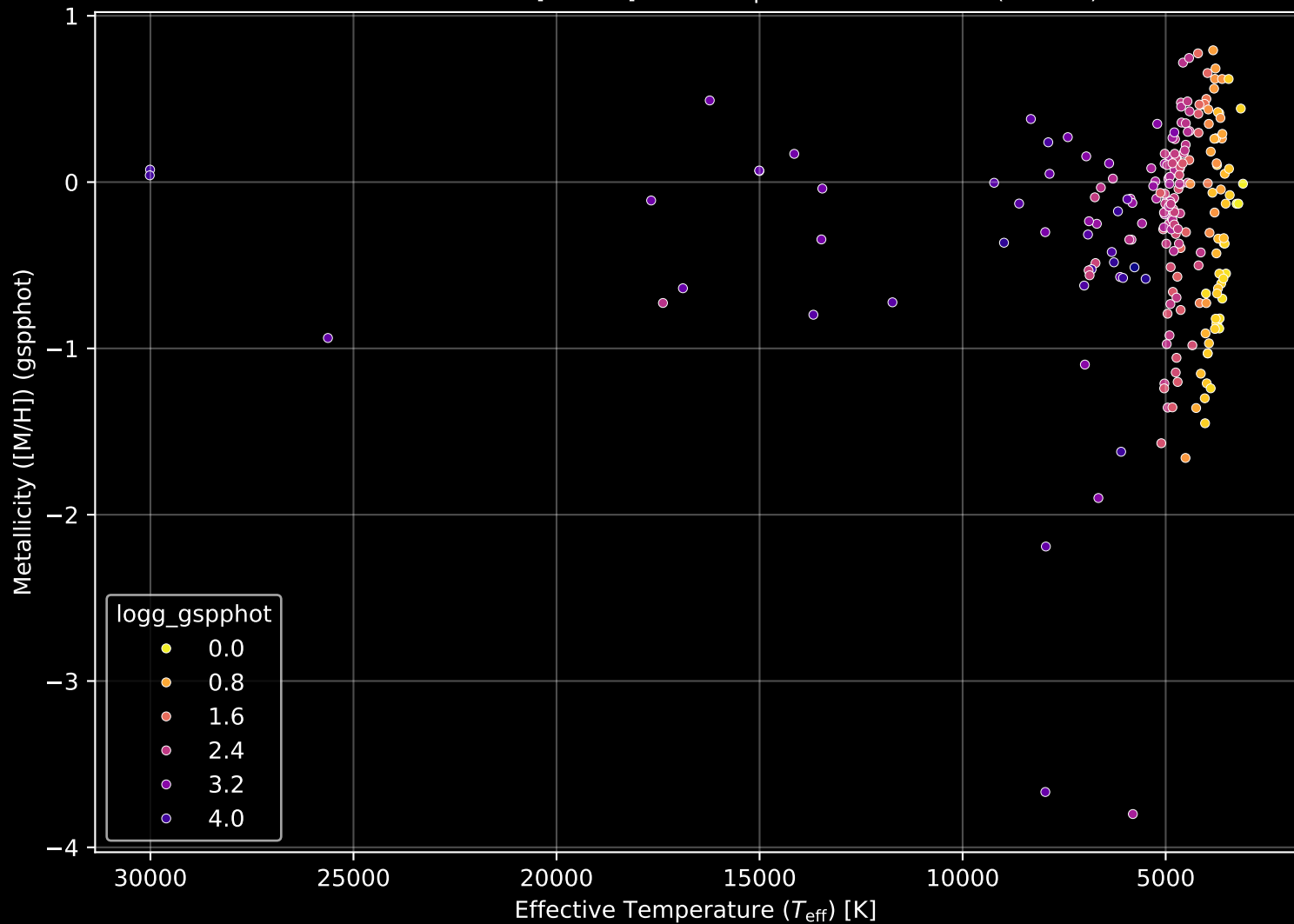
APOGEE DR17 Field: [006-02] Stellar Population Parameters (n= 225)
