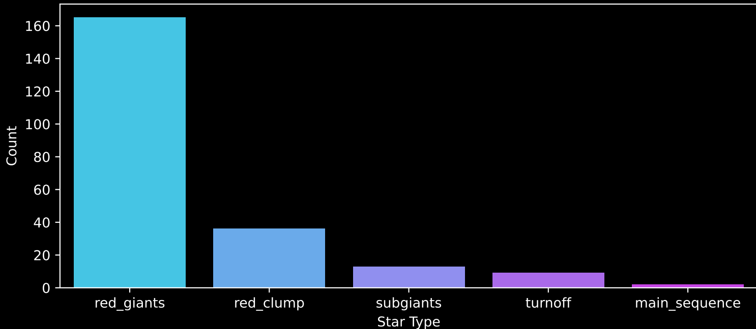
APOGEE DR17 Field: [006-02] Count plot of Star Type
