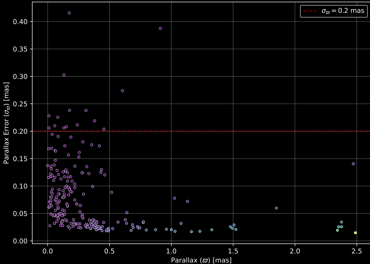
APOGEE DR17 Field: [006-02] Parallax Quality (n= 225)
